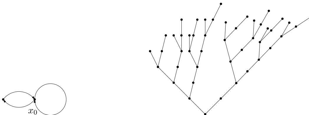
Figure 2.2. A graph and part of its directed cover. This tree is also called the Fibonacci tree .
