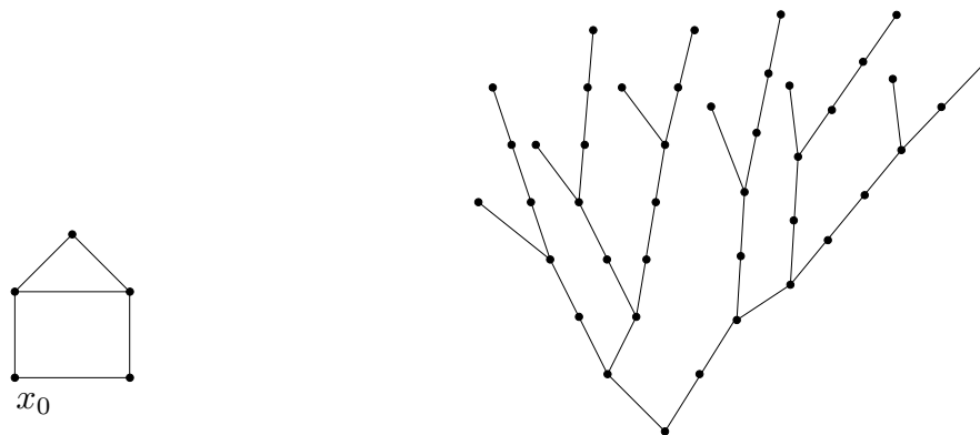
Figure 2.1. A graph and part of its universal cover.
