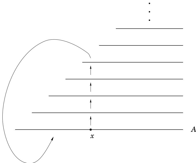
Figure 11.2. A schematic of a tower over A , showing part of an orbit of x .
