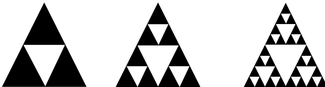
Figure 12.1. The first three stages of the construction of the Sierpinski gasket.
