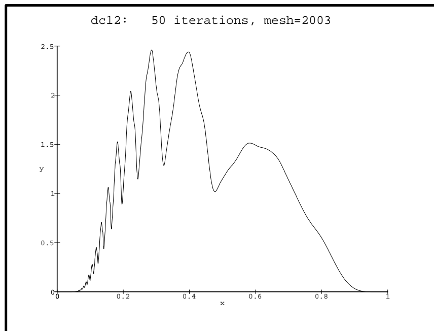
Figure 11.1. The apparent density of the conductance for p_1 = p_2 = 1/2 .
