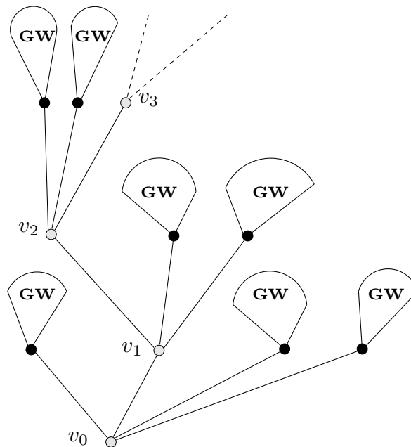
Figure 10.1. Schematic representation of size-biased Galton-Watson trees.
