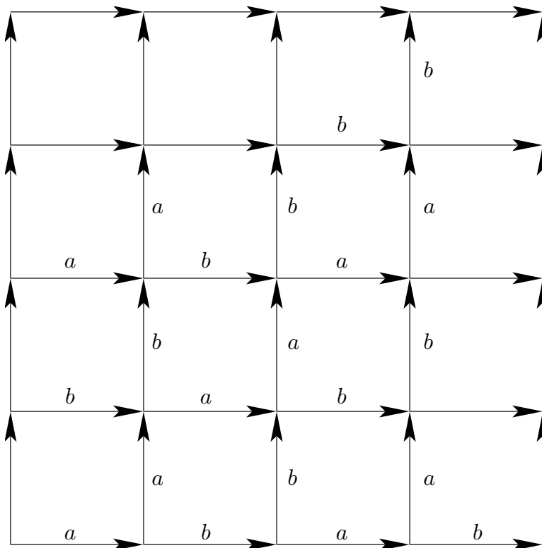
Figure 6.1. A portion of the edge-labelled Cayley graph of \mathbb{Z} *_\mathbb{Z} \mathbb{Z} .
