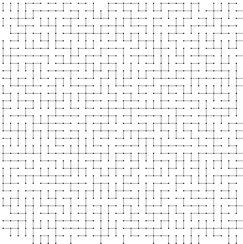
Figure 8.2. A portion of a uniformly chosen spanning tree on \mathbb{Z}^2 , drawn by David Wilson.
