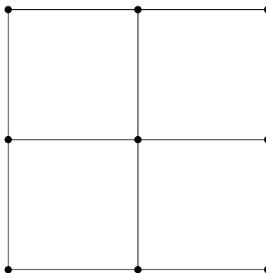
Figure 5.1. The simplest case.
