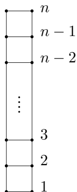
Figure 1.8. A ladder graph.
