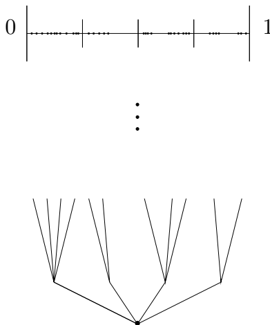
Figure 12.3. In this case b = 4 .
