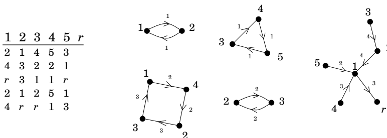
Figure 8.1. This Markov chain has 6 states, one called r , which is the root. The first 5 elements of each stack are listed under the corresponding states. Colored cycles are popped as shown clockwise, leaving the colored spanning tree shown.
