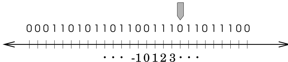
Figure 6.2. A typical element of G_1 .
