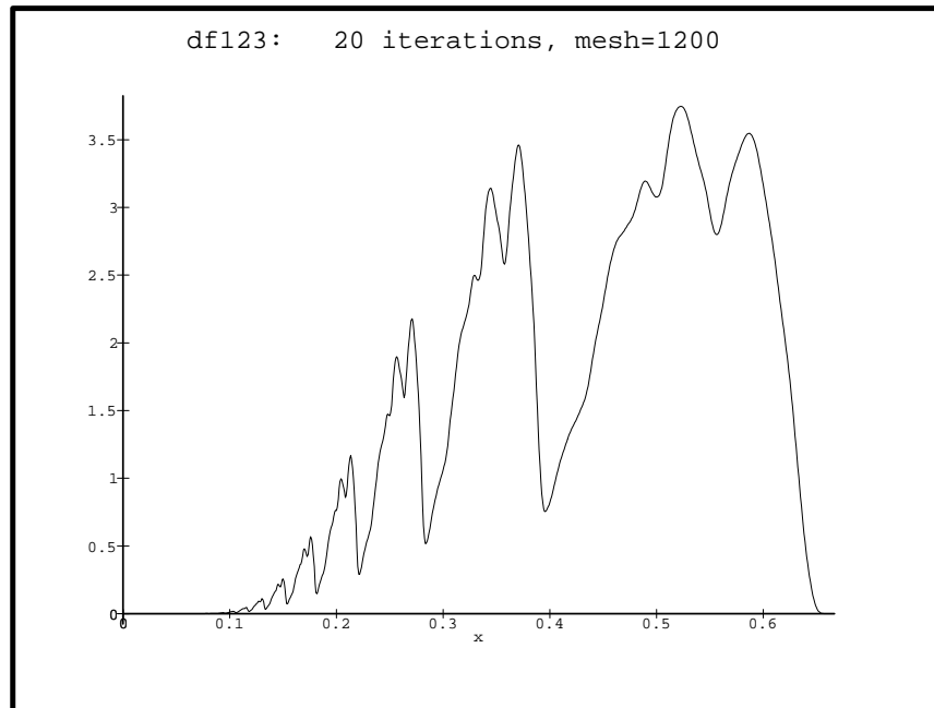
Figure 14.3. The apparent GW -density of \gamma(T) for f(s) = (s + s^2 + s^3)/3 .
