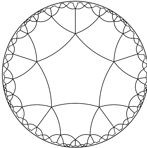
Figure 2.4. A Cayley graph in the hyperbolic disc formed from regular hyperbolic pentagons of interior angle 2\pi/5 .
