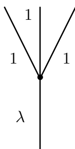
Figure 1.6. The relative weights at a vertex. The tree is growing upwards.
