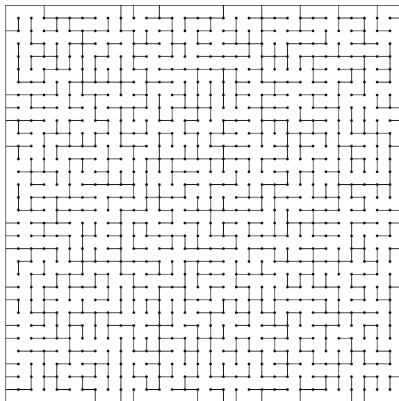
Figure 9.1. A uniformly chosen wired spanning tree on a subgraph of \mathbb{Z}^2 , drawn by Wilson (see Propp and Wilson (1998)).
