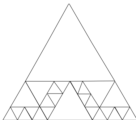
Figure 12.5. The sets I_v for the top side of the von Koch snowflake.
