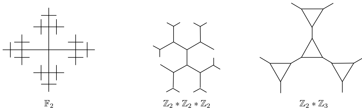
Figure 2.3. Some Cayley graphs.
