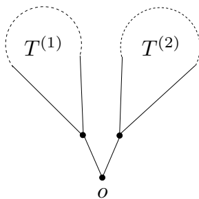
Figure 1.3. Joining two trees.
