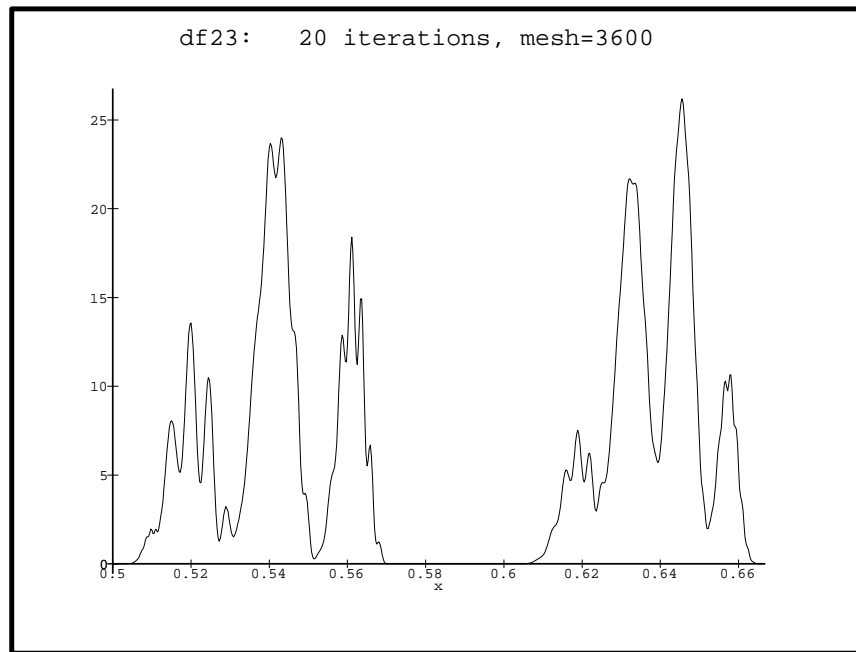
Figure 14.2. The apparent GW-density of \gamma(T) for f(s) = (s^2 + s^3)/2 .
