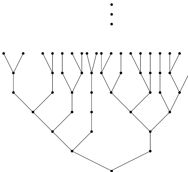
Figure 4.1. A typical Galton-Watson tree for f(s) = (s + s^2)/2 .
