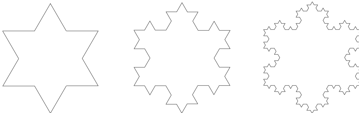
Figure 12.4. The first three stages of the construction of the von Koch snowflake.
