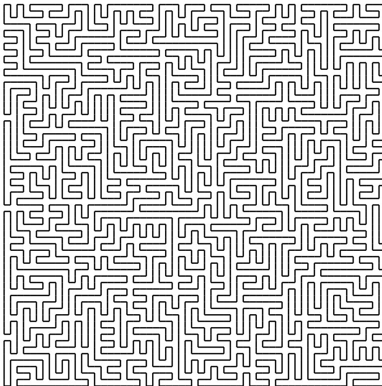
Figure 9.3. The inside of this lattice-filling curve is a uniform spanning tree on a square grid, while the outside is another on the dual grid (wired).
