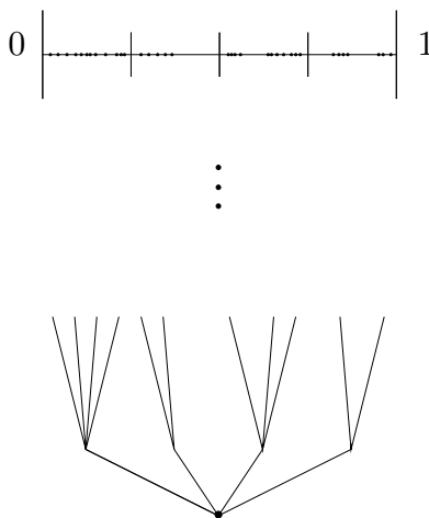
Figure 1.11. In this case b = 4 .
