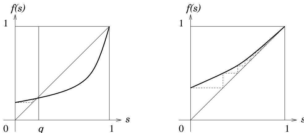
Figure 4.2. Typical graphs of f when m > 1 and m \leq 1 .
