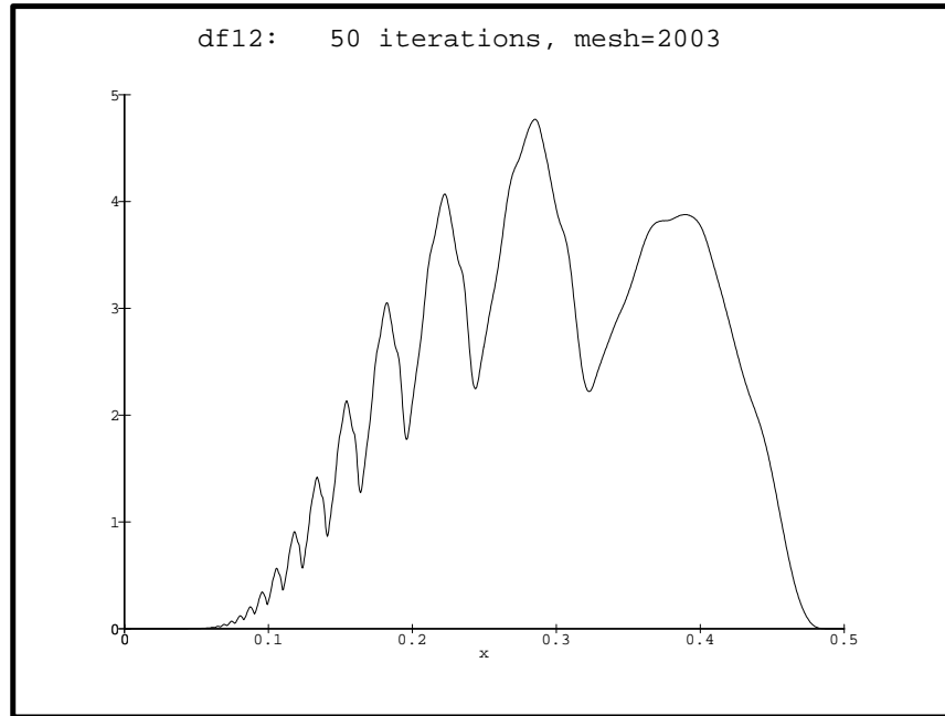
Figure 14.1. The apparent GW-density of \gamma(T) for f(s) = (s + s^2)/2 .
